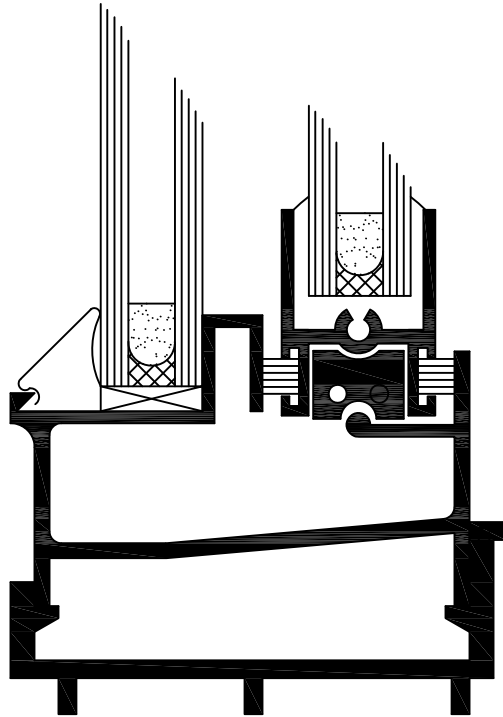
22 SERIES 501 COMPENSATION CHANNEL HEAD/JAMB SIMILAR
