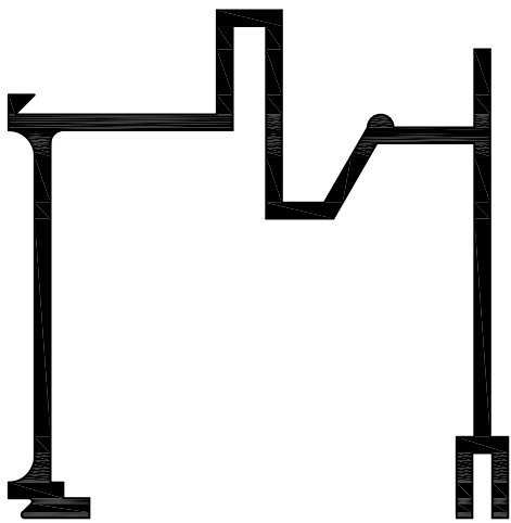
HIGH WATER SILL FOR C 40 RATING
